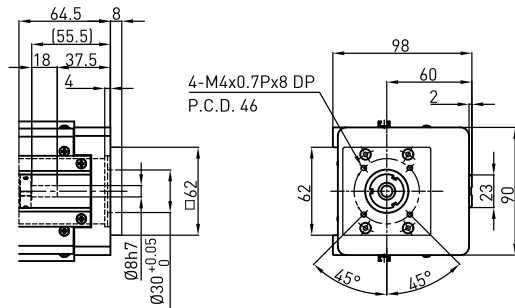
Motor Adaptor Flange F2
