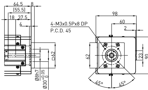
Motor Adaptor Flange F5
