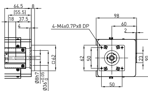
Motor Adaptor Flange F6
