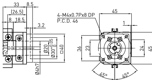
Motor Adaptor Flange F2
